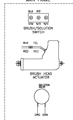
MAIN FRAME
