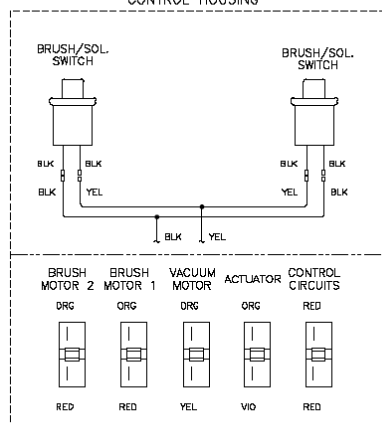
CONTROL HOUSING
