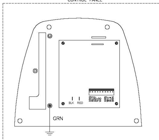
CONTROL PANEL
